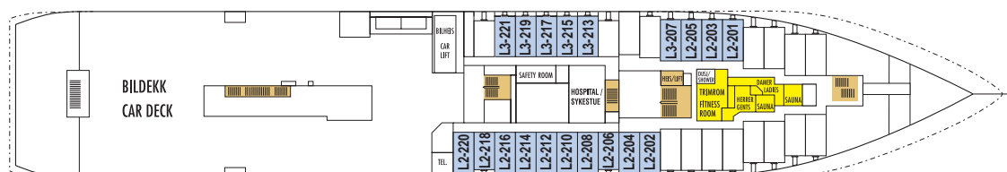
DECK 2
